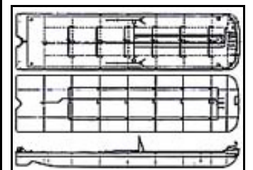
TB99041 Tank Barge
