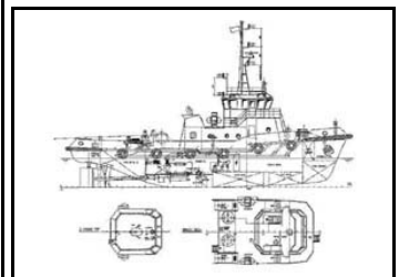
TG30035 Twin Screw Tug
