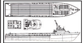
CB18336 Crew Boat
